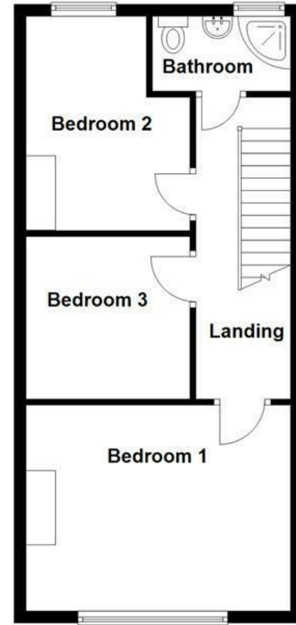
First Floor Approx. 44.9 sq. metres (482.9 sq. feet)
